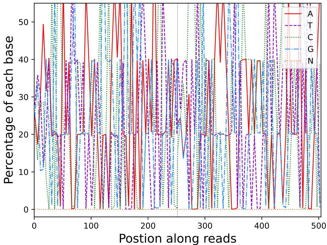
Base percentage along reads (R20123)
